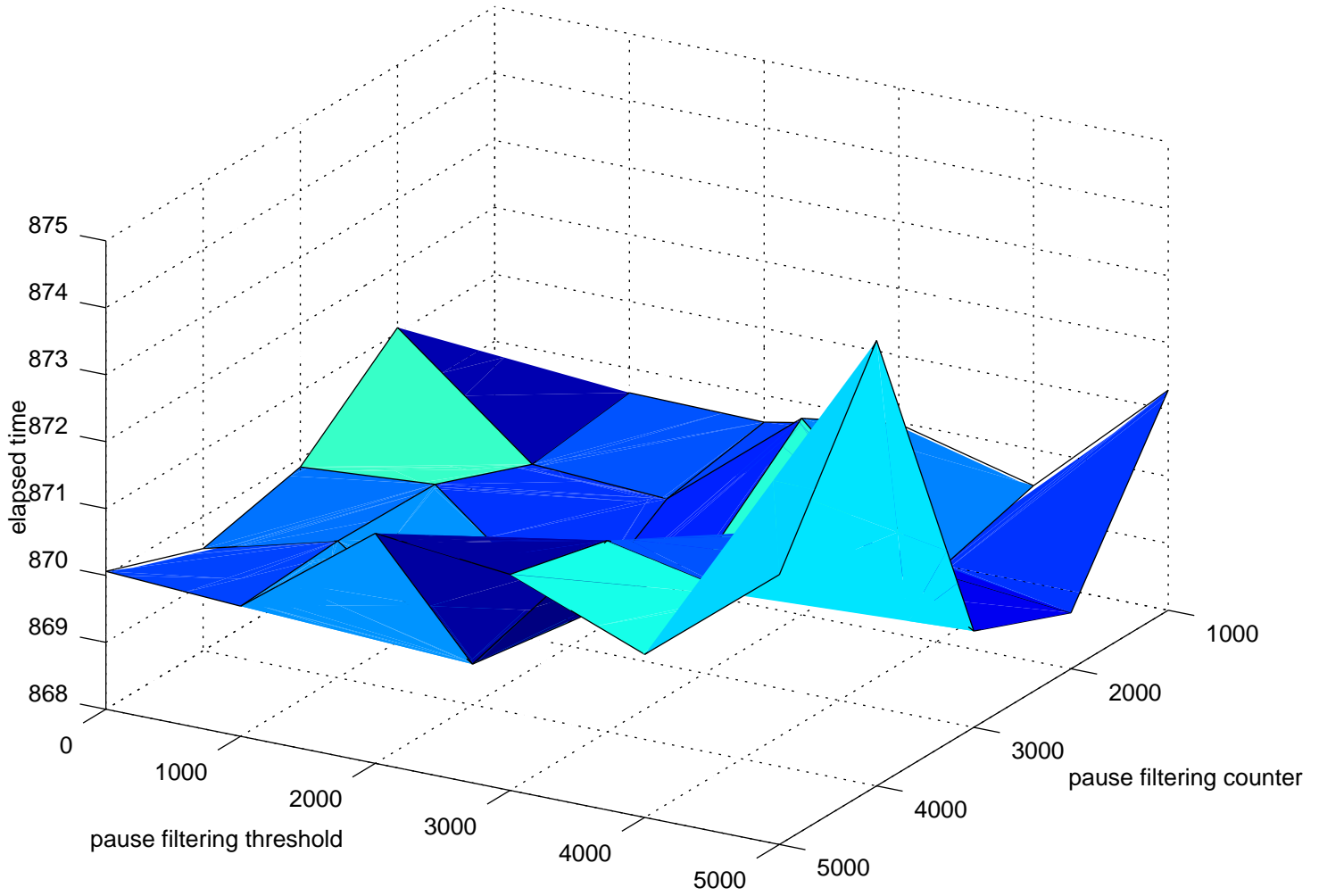
Elapsed time in -j cpucount/2 kernbench vs pause variables
